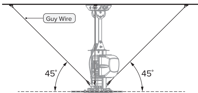
Fig. 2.1: Side View (X-Y)
