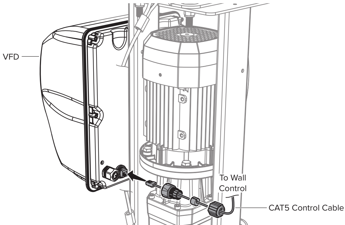
Fig. 1: CAT5 Control Cable to VFD
