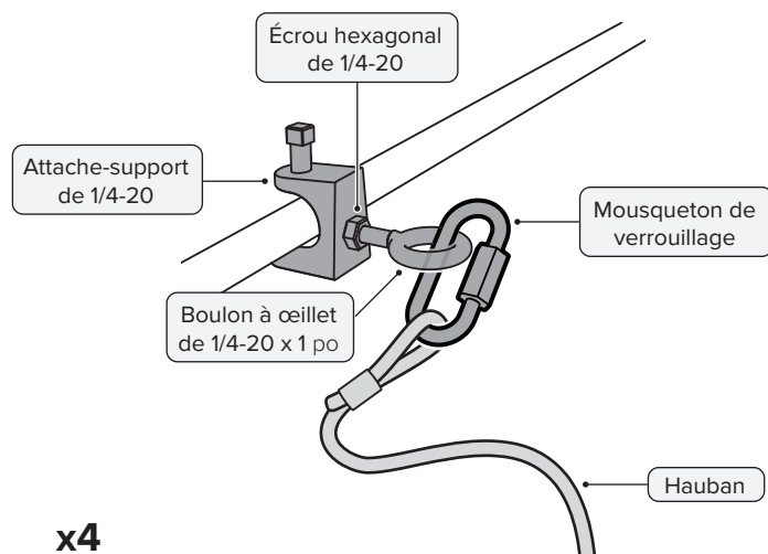
Fig. 2.3 : Attaches-supports
