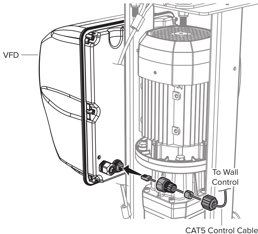
Fig. 1: CAT5 Control Cable to VFD
